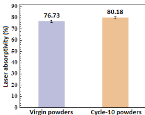
Fig. S1 Comparison between laser absorptivity values of LPBF-fabricated NiTi specimens made from virgin powders and Cycle-10 powders.
