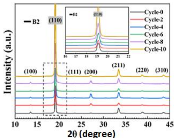
Fig. S2 XRD patterns of LPBF-fabricated NiTi specimens made from virgin powders and reused powders (collection temperature: 100 °C).
