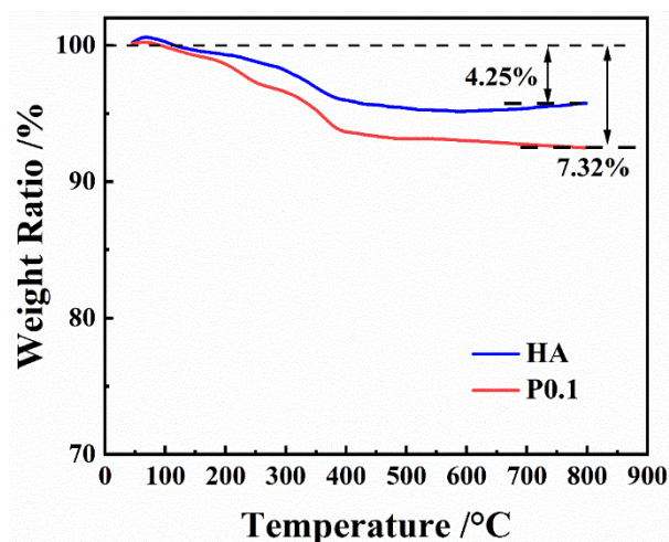
Fig. S2 Thermal decomposition curves of samples HA and P0.1.
