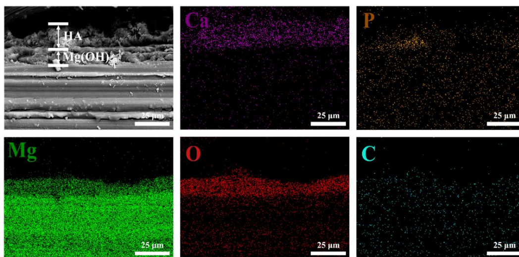
Fig. S1 SEM images of the cross-section of the HA/PA composite coating and elemental distributions.
