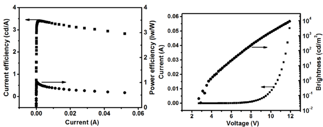
Figure 1S device performance, left, current efficiency vs current characteristics. Right, Current-voltage-Brightness characteristics.
