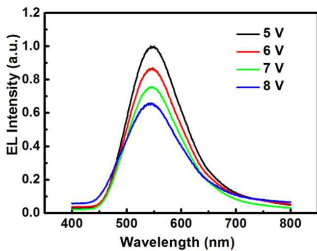
Figure 2S EL spectrum at various voltages.
