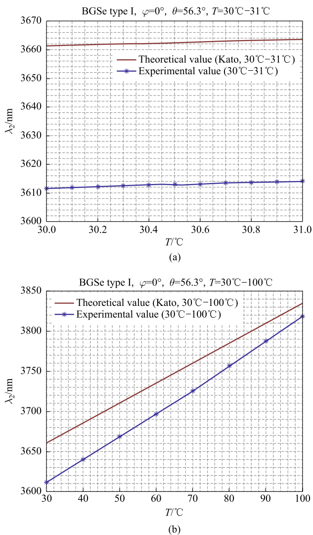
Fig. 6 Relationship between output wavelength and temperature rose a from 30 ^{\circ}\text{C} to 31 ^{\circ}\text{C} , and b from 30 ^{\circ}\text{C} to 100 ^{\circ}\text{C}
