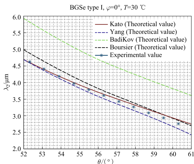
Fig. 3 Relationship between BGSe OPO idler wavelength and angle
