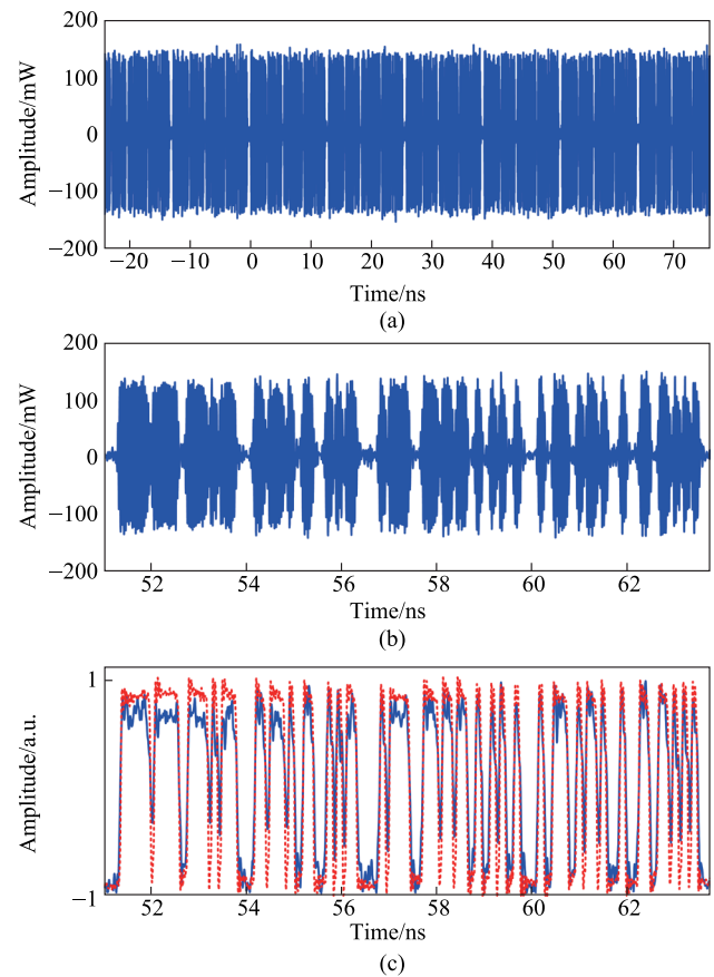
Fig. 4 Measured results of the photonic generated microwave signal when the frequency interval between CW1 and CW2 is 30 GHz and the bit rate of the PRBS coding signal is 10 Gb/s. a Temporal waveform of the generated microwave SSB signal after the EA. b Zoomed-in view of the temporal waveform in one coding period (from 51.05 to 63.75 ns). c Recovered coding signal (blue solid curve) and the original PRBS driving signal (red dashed curve)
