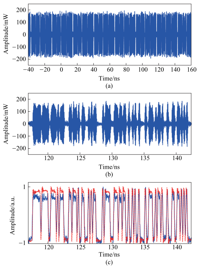
Fig. 5 Measured results of the photonic generation of microwave signal when the frequency interval between CW1 and CW2 is 20 GHz and the bit rate of the PRBS coding signal is 5 Gb/s. a Temporal waveform of the generated microwave SSB signal after the EA. b Zoomed-in view of the temporal waveform in one coding period (from 116.95 to 142.25 ns). c Recovered coding signal (blue solid curve) and the original PRBS driving signal (red dashed curve)
