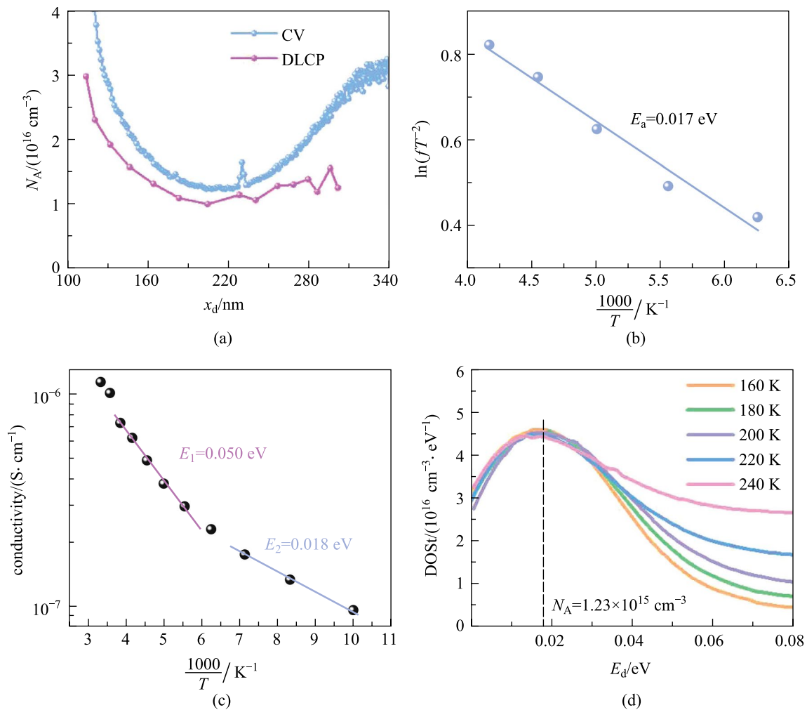
Fig. 4 a Relationship between N_A and x_d measured by C–V and DLCP. b Arrhenius plot. c Temperature dependent dark-state conductivity. d Defect DOS
