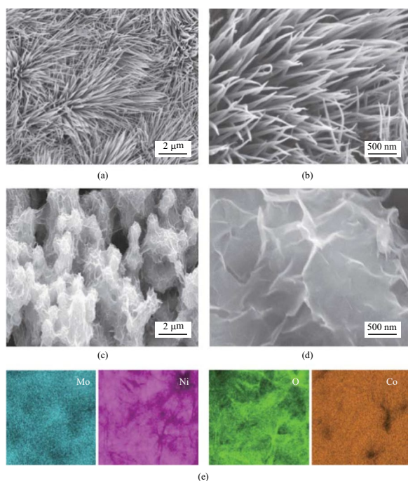
Fig. 2 Morphology characterization. a and b \text{Co}_3\text{O}_4 samples. c and d \text{Co}_3\text{O}_4@\text{NiMoO}_4 samples. e Elemental mappings
