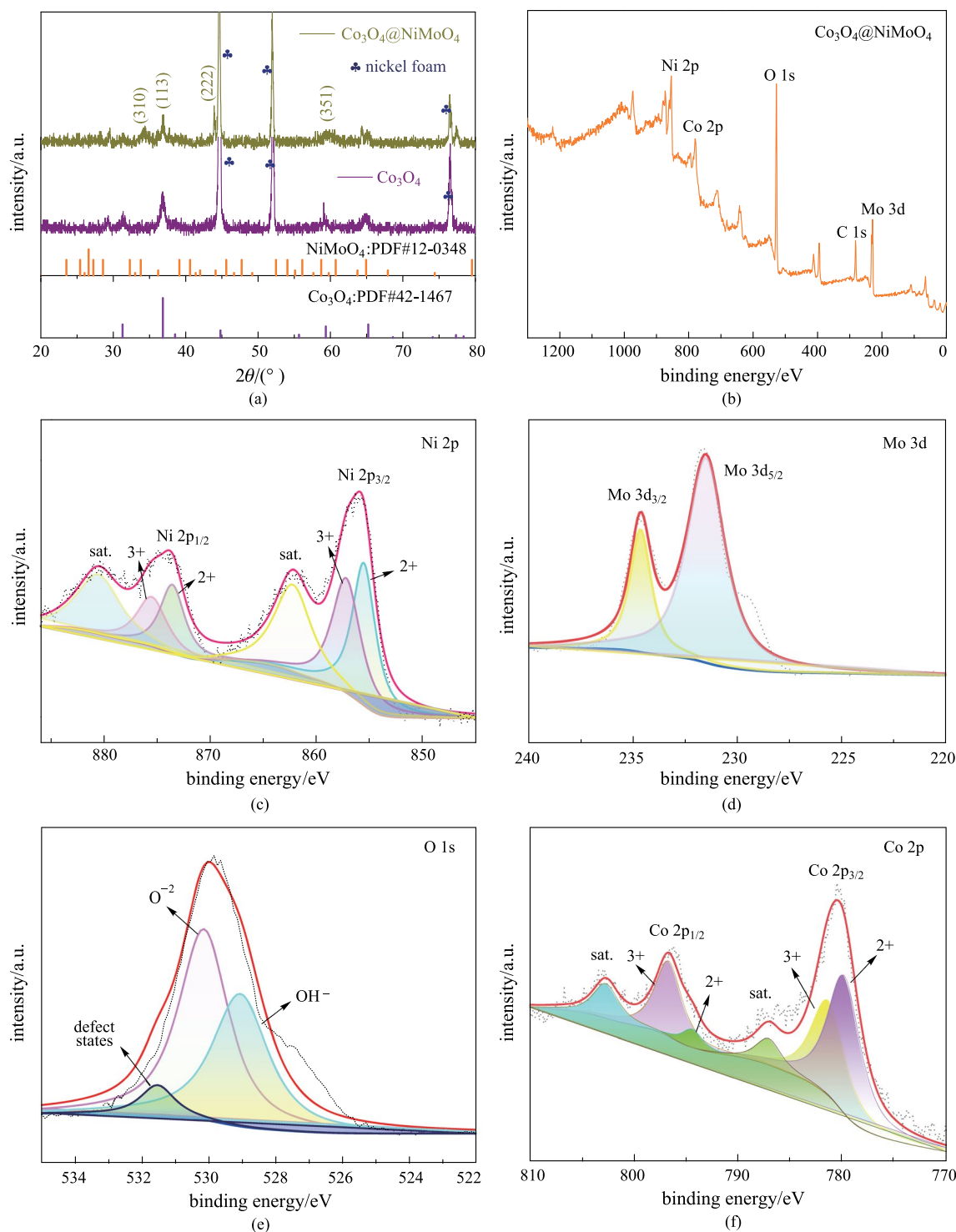
Fig. 3 a XRD patterns of the samples. b Full spectra of XPS spectra of \text{Co}_3\text{O}_4@\text{NiMoO}_4 . Samples c Ni 2p, d Mo 3d, e O 1s, and f Co 2p
