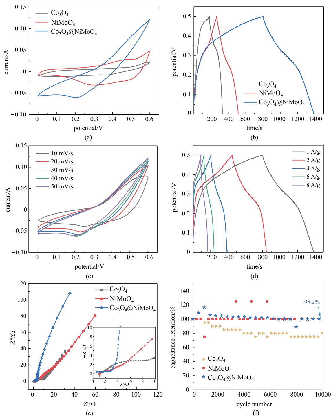
Fig. 4 a CV curves at 50 mV/s. b GCD curves at 1 A/g. c CV curves. d GCD curves. e Nyquist plots. f Cycle performance
