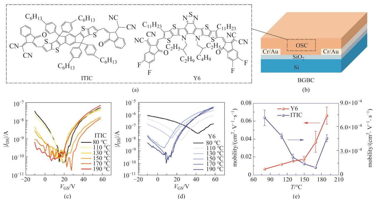
Fig. 1 Basic characterization of Y6 and ITIC TFTs. a Molecule structure of ITIC and Y6. b Schematic diagram of the BGBC device used in this study. Here the OSC indicates organic semiconductor. The transfer characteristics of c ITIC and d Y6 BGBC devices with semiconductor films annealed at different temperatures ( V_{\text{DS}} = 60\text{ V} ). e Extracted mobility of the two devices as a function of annealing temperature
