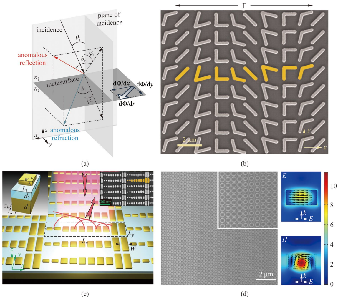
Fig. 1 Pioneer works demonstrating the fundamental design rules. a Schematics of the generalized Snell's law of reflection and refraction. The gradient of phase shift d\Phi/dr at the interface offers an effective wavevector that can bend reflected and transmitted light in designed directions. b Scanning electron microscope (SEM) image of the plasmonic metasurface with V-shaped optical antennas. c Schematic of the reflect-array metasurface with gold patch antennas separated from a gold substrate by a dielectric spacer with subwavelength thickness. The left inset shows a schematic of an individual unit-cell, and the right inset is the corresponding SEM image of the metasurface. d SEM image of a dielectric metasurface Huygens' beam deflector and the corresponding simulated field distributions. a Reprinted with permission of IOP Publishing, from Ref. [23]; permission conveyed through Copyright Clearance Center, Inc. [13]. Copyright 2011, The American Association for the Advancement of Science. c Reprinted with permission from Ref. [24]. Copyright 2012, American Chemical Society. d Reprinted with permission from Ref. [25]. Copyright 2015, WILEY-VCH Verlag GmbH & Co. KGaA, Weinheim
