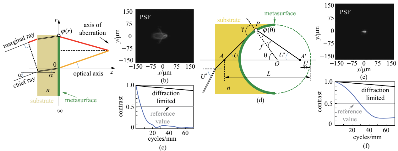
Fig. 9 Aplanatic metalens. a A flat metalens illuminated by parallel rays incident at angle \alpha . The OPD equals the red segment plus the equivalent OP of phase discontinuity \frac{\lambda}{2\pi}\phi(r) , subtracting the yellow segment. b Point spread function (PSF) and c modulation transfer function (MTF) of flat metalens. d Schematics of an aplanatic metalens with metasurface pattern on a spherical substrate. e PSF and f MTF of aplanatic metalens. The sidelobe here is significantly reduced compared with b . And the spatial resolution at minimum contrast 0.5 is enhanced from 8 to 30 cycles/mm. a–f Reprinted with permission from Ref. [80]. Copyright 2013, The Optical Society
