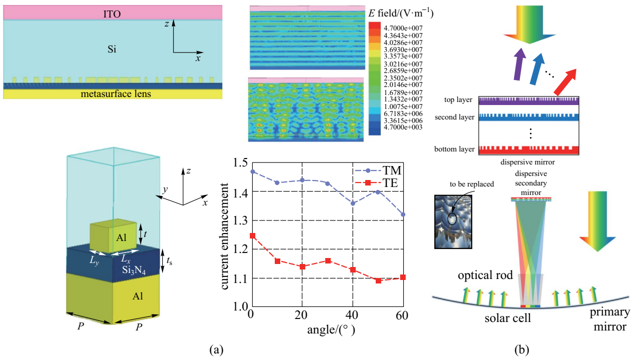
Fig. 19 Applications in solar energy harvesting. a Metasurface lens integrated into a silicon solar cell to enhance light absorption by trapping light into the active area. The simulated result shows field enhancement at 550 nm incident wave which is TE polarized. The short circuit current exhibits improvement at angles up to 60°. b Multi-layer dielectric high-index-contrast gratings (HCG). Normally incident lights are directed to different angles depending on wavelengths. By replacing the secondary mirror, the HCG dispersive mirror can act as both sunlight concentrator and spectral splitter. a Reprinted with permission from Ref. [116]. © The Optical Society. b Reprinted with permission from Ref. [115]. Copyright 2014, Springer-Verlag Berlin Heidelberg
