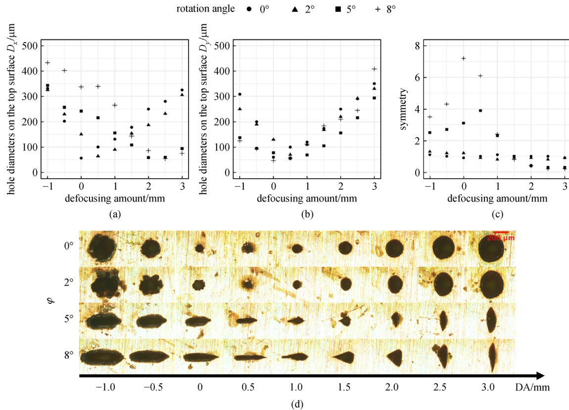
Fig. 5 Dependences of the top-surface hole diameters D_x (a), D_y (b), and symmetry (c) on the lens rotation angle and target defocusing amount. (d) Optical microscopic images of holes on the top target surface. The copper plate has a thickness of 0.5 mm. These through-holes are drilled by femtosecond laser with an average power of 0.5 W
