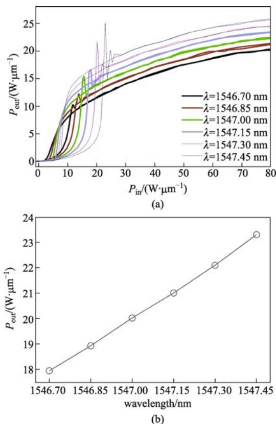
Fig. 5 (a) P_{\text{out}} as a function of P_{\text{in}} for \lambda = 1546.70 to 1547.45 nm; (b) dependence of P_{\text{out}} on the wavelength for P_{\text{in}} = 55 W/ \mu\text{m} (in the range of P_{\text{in}} > 30 W/ \mu\text{m} )
