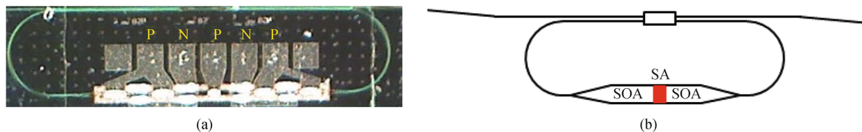
Fig. 6 (a) Photograph of the ring cavity colliding pulse mode-locked laser. The letters are added for clarity and denote the P and N contacts for the centered absorber and the two gain sections on either side; (b) schematic of the gain, absorber and waveguide sections inside the laser cavity. SA-saturable absorber, SOA-semiconductor optical amplifier
