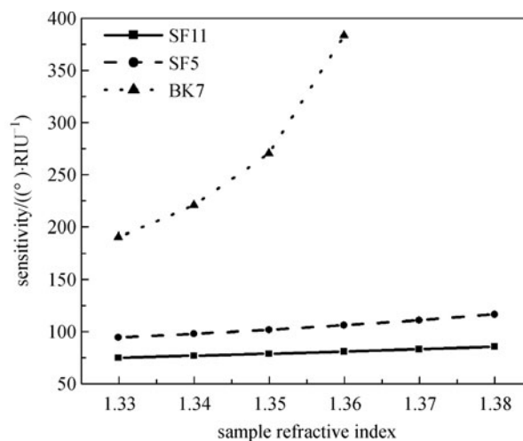
Fig. 5(e) Sensitivity vs. sample refractive index plot for three prism materials
