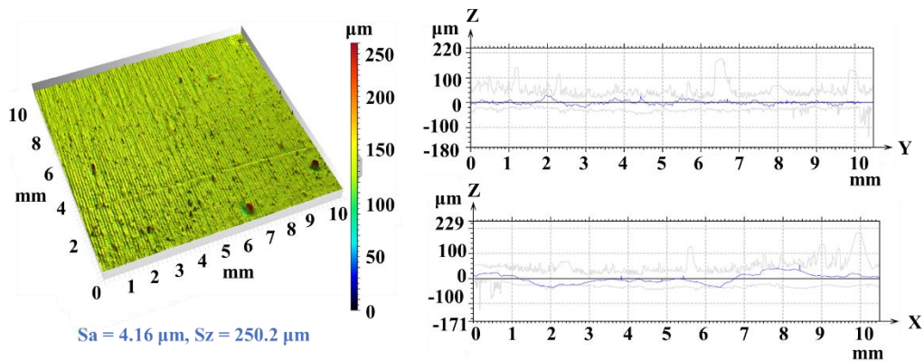
Fig. S1 3D surface profile of as-SLMed surface with an area of 10.49 \text{ mm} \times 10.49 \text{ mm} .
