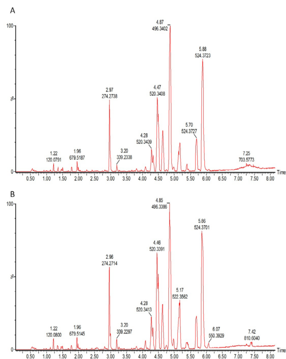
Fig. S1 The CON rat serum chromatogram (A) and MOD rat serum chromatogram (B) which acquired by UPLC-MS-Q-ToF.
