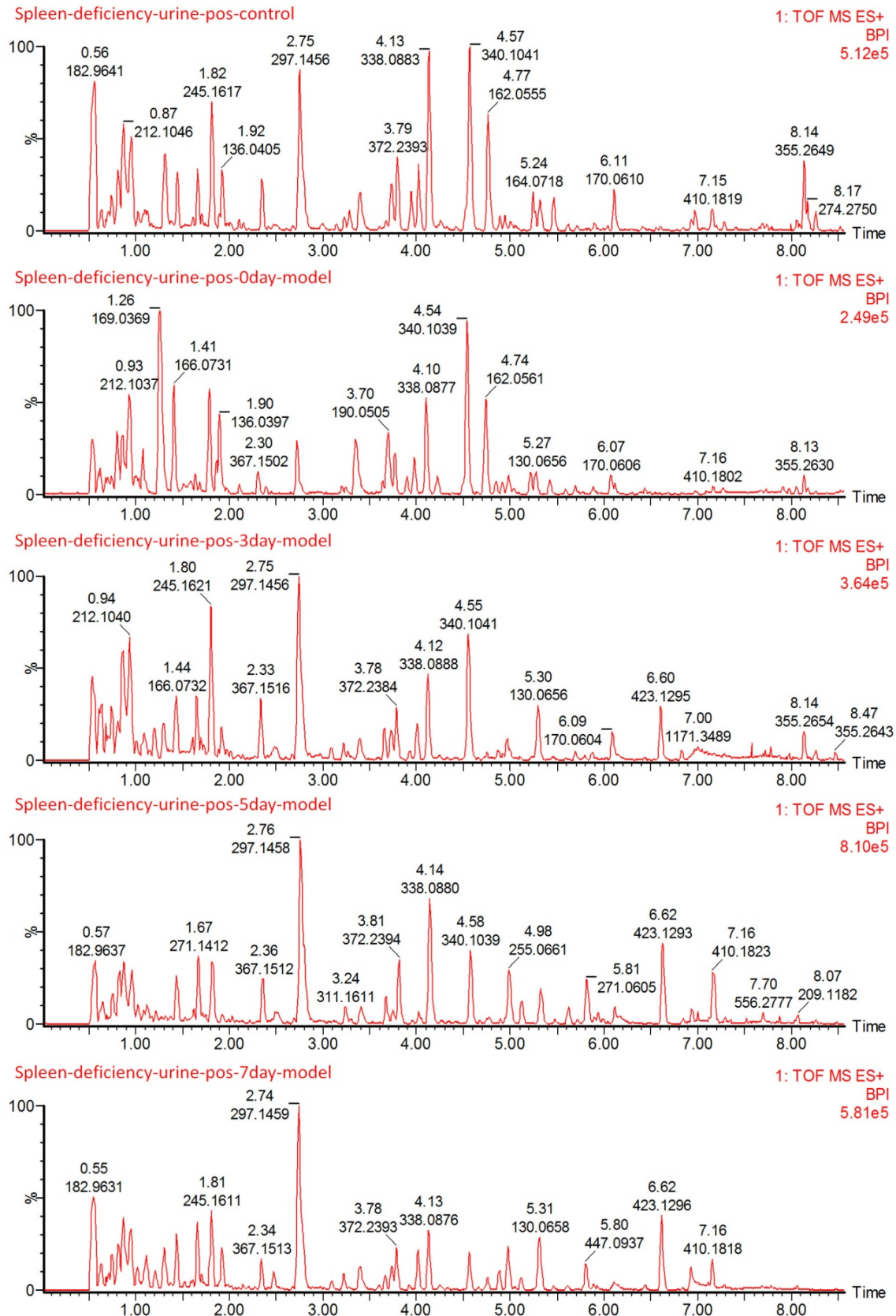
Fig. S2 The CON rat urine chromatogram, the 0, 3, 5, 7days MOD rat urine chromatogram (in proper order which from up to down) which acquired by UPLC-MS-Q-ToF.
