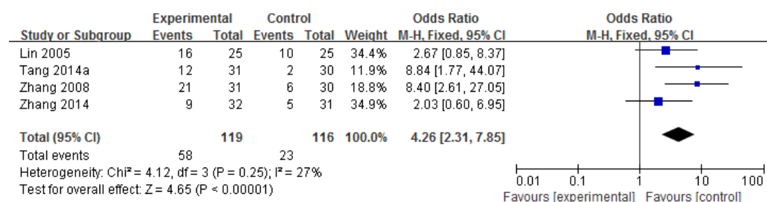
Fig.11 A forest plot of Meta-analysis of 2-year survival rates (studies with unclear risk of bias)
