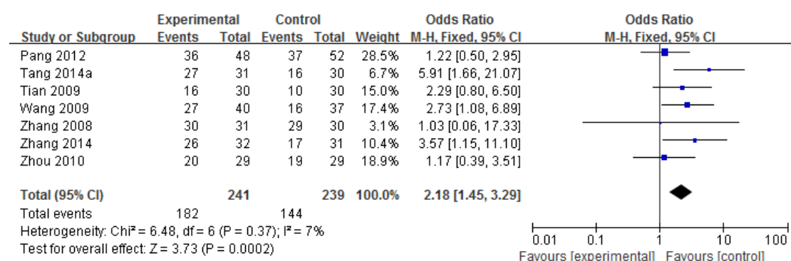
Fig. 7 A forest plot of Meta-analysis of half-a-year survival rates (studies with unclear risk of bias)
