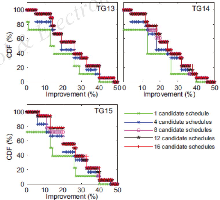
Fig. 14 The CDF of chips over the improvement of results achieved by HASR and DTS against base performance for real applications with different candidate schedule quantities
