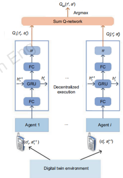
Fig. 3 The MARL method for the DT deployment structure (MARL: multi-agent reinforcement learning; DT: digital twin; GRU: gate recurrent unit; FC: fully connected)
