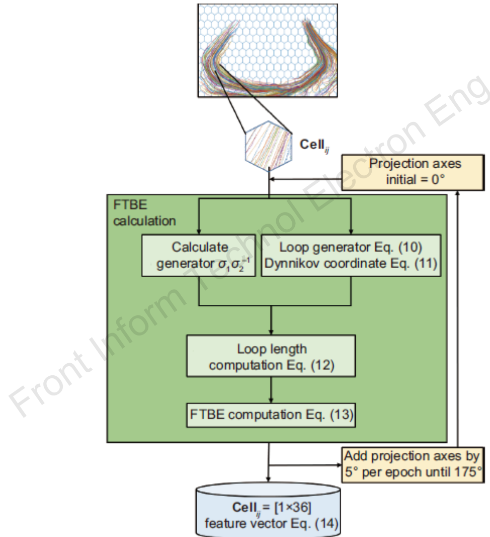
Fig. 5 Calculating the feature vector for each cell using braid entropy
