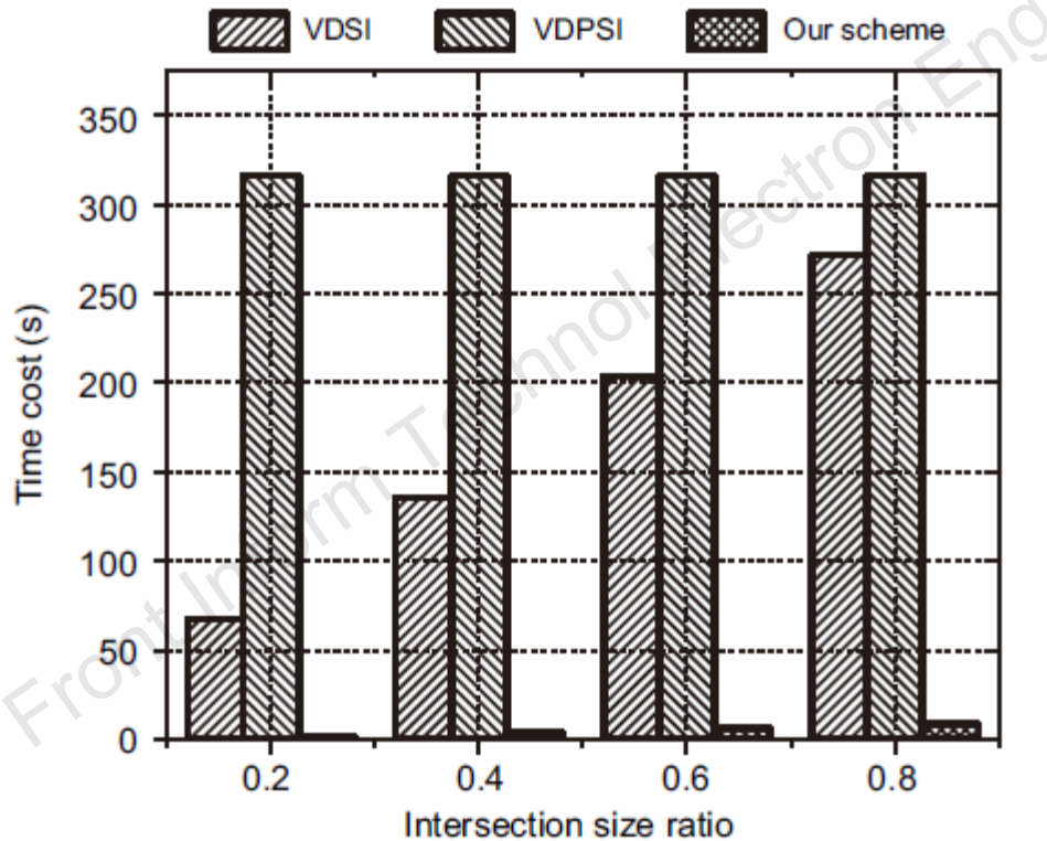
Fig. 3 Computation cost at dataset size n = 32\,768
