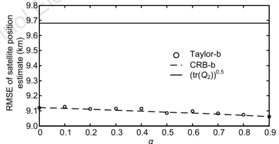
Fig. 8 RMSEs of satellite position estimates versus \alpha
