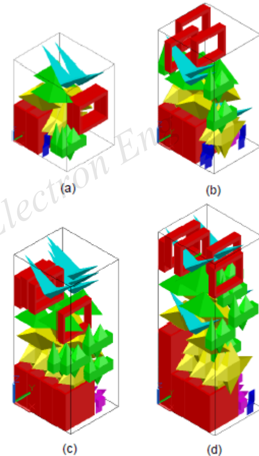
Fig. 13 Layout generated using HAPE3D when rotation is forbidden (RN=1)
