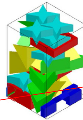
(b) HAPE3D+SA (500 iterations) h=31.2 mm t=9637.5 s
