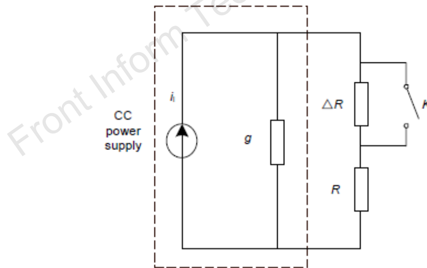
Fig. 2 Diagram for system identification of power supply (CC: constant current)
