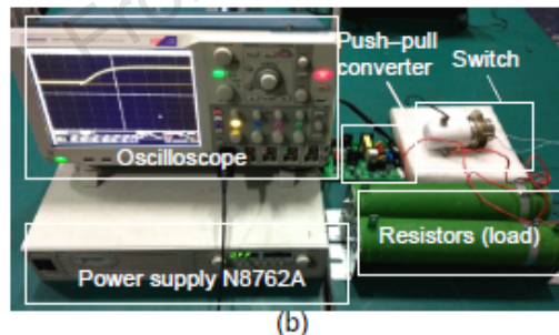
Fig. 7 The experimental schematic for \alpha adjustment (a) and the corresponding setup of the experiment (b) (CC: constant current)
