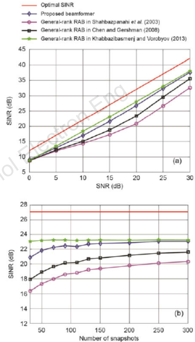
Fig. 1 Output SINR versus SNR (a) and the number of snapshots (b)
