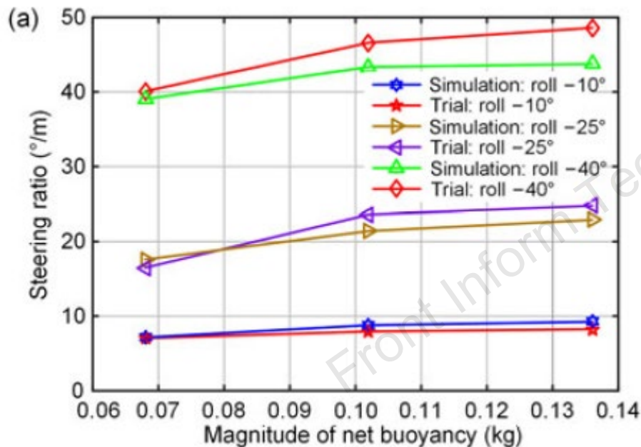
Fig. 12 Steering ratio for simulation and trial of cases A-1–A-9 (a) and cases B-1–B-3 (b)
