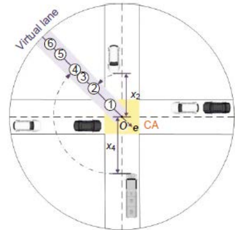
One-dimensional (1D) virtual platoon
