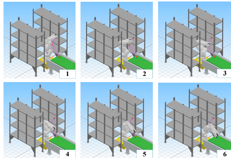
Fig. 15 Motion process of simulation case
