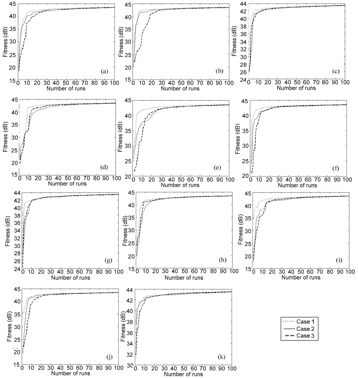
Fig. S2 Values of fitness of GA-IPM-2-GA-IPM-12 ((a)–(k), respectively) for 100 independent runs for problem 1
