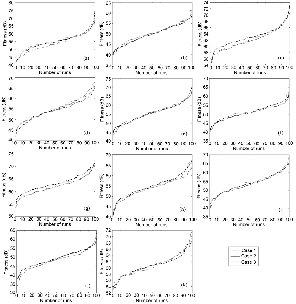
Fig. S3 Results of GA-2–GA-12 ((a)–(k), respectively) for 100 independent runs based on values of fitness for problem 2
