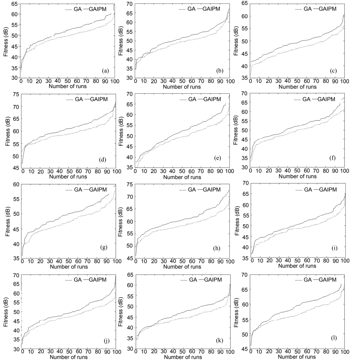
Fig. S5 Values of fitness of GA-1–GA-12 ((a)–(l), respectively) for 100 independent runs for problem 3
