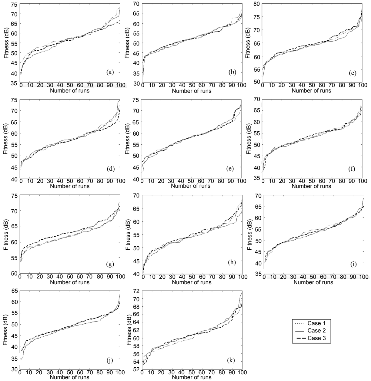
Fig. S4 Values of fitness of GA-IPM-2-GA-IPM-12 ((a)–(k), respectively) for 100 independent runs for problem 2
