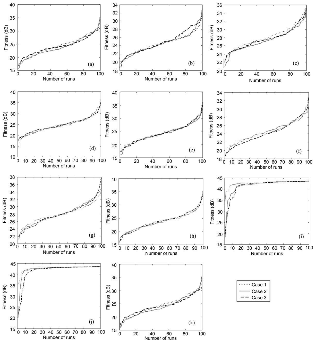
Fig. S1 Results of GA-2-GA-12 ((a)–(k), respectively) for 100 independent runs based on fitness for problem 1
