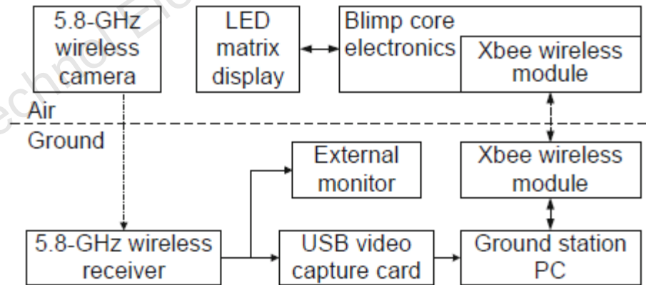
Fig. 3 Hardware overview
