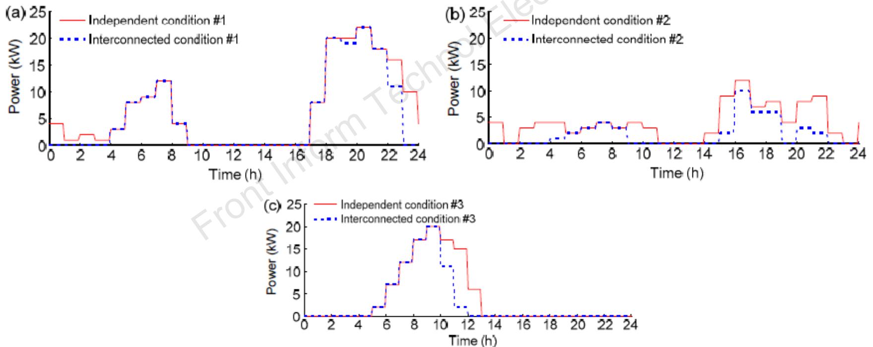
Fig. 10 Curves of the controllable power supply in independent and interconnected conditions of microgrids #1 (a), #2 (b), and #3 (c)
