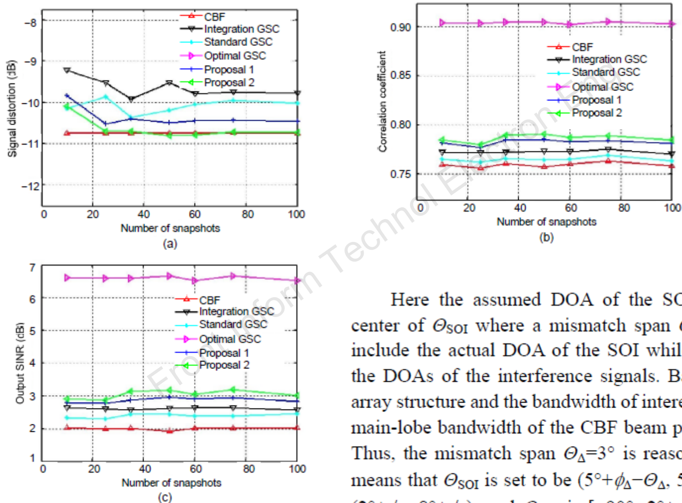
Fig. 2 Performance measurements in terms of the number of snapshots with SNR=-10 dB: (a) signal distortion; (b) correlation coefficients with the SOI; (c) output SINR
