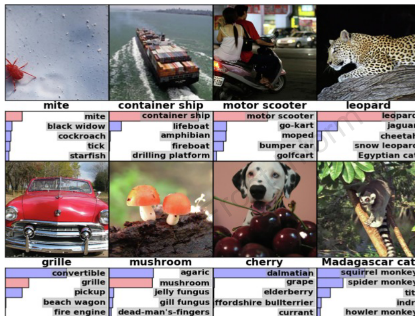
Image classification
