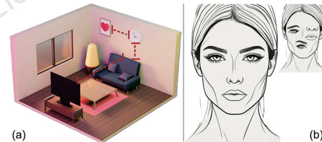
Geometric relations
