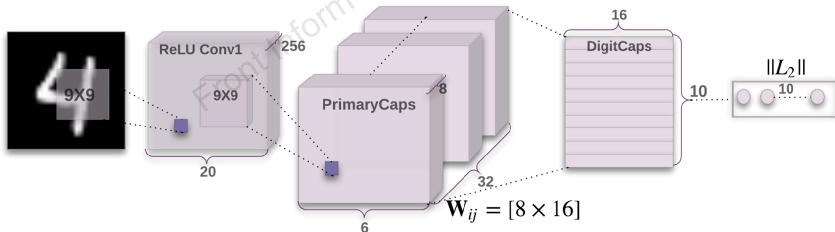
Capsule network
