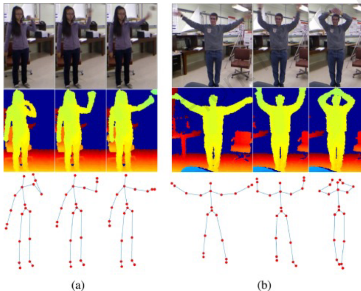
Action recognition
