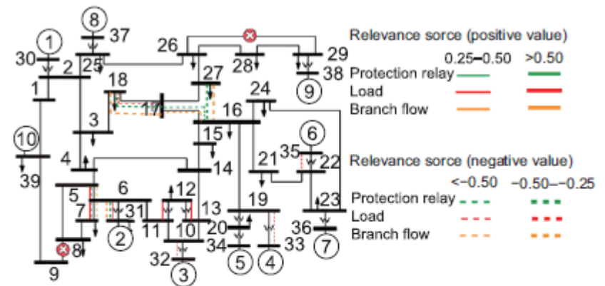
Fig. 9 Topological graph representing a part of IEEE 39 after L16 and L44 are triggered. The target class is predicted as a medium-level component outage. References to color refer to the online version of this figure
