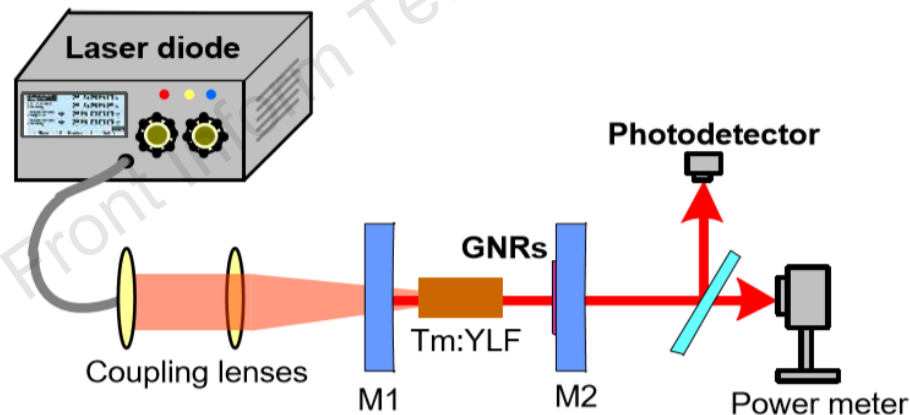
Fig. 1 Sketch of the LD-pumped Tm:YLF laser used in this analysis
