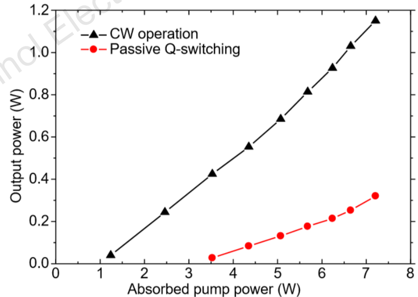
Fig. 3 Output power and absorbed LD pump power
