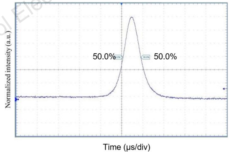
Fig. 6 Shape of the 843 ns pulse
