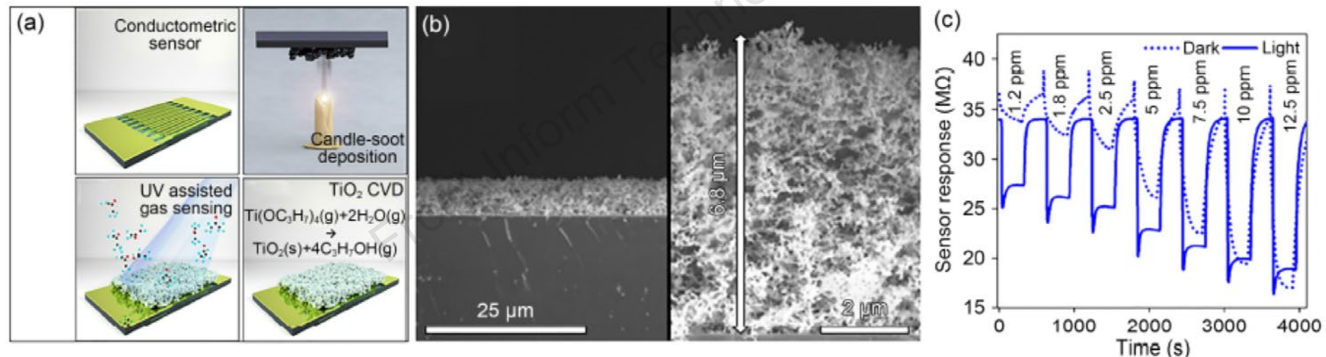
Fig. 5 Schematic of the fabrication process of a soot template \text{TiO}_2 gas sensor (a), different magnification scanning electron microscope (SEM) images showing the uniformity and thickness of the surface of a \text{SnO}_2 sensor device (b), and dynamic response curve of the \text{SnO}_2 gas sensor to different acetone concentrations (c)
