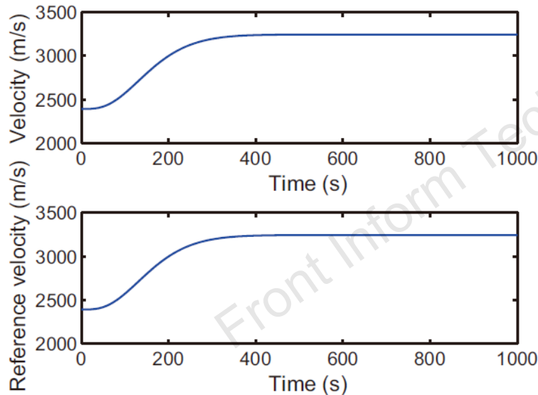
Fig. 2 Velocity tracking
