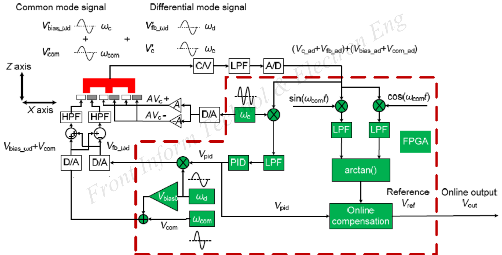
Fig. 5 Novel closed-loop diagram with a modulated feedback approach and temperature compensation
