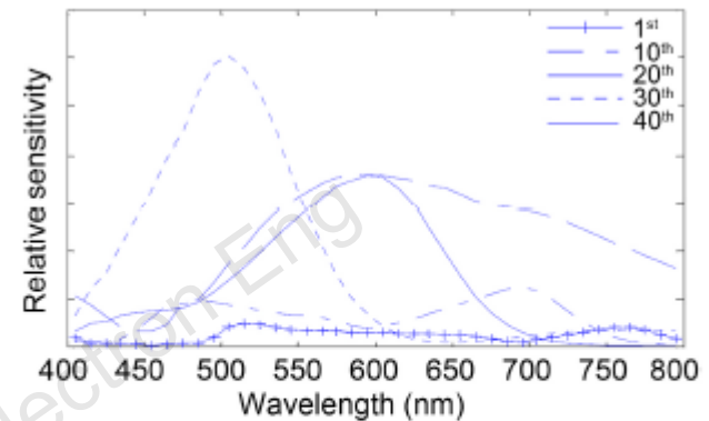
Fig. 8 Sensitivity responses of five spectral detectors among 40 low-cost filters Reprinted from Chang and Lee (2008), Copyright 2008, with permission from OSA
