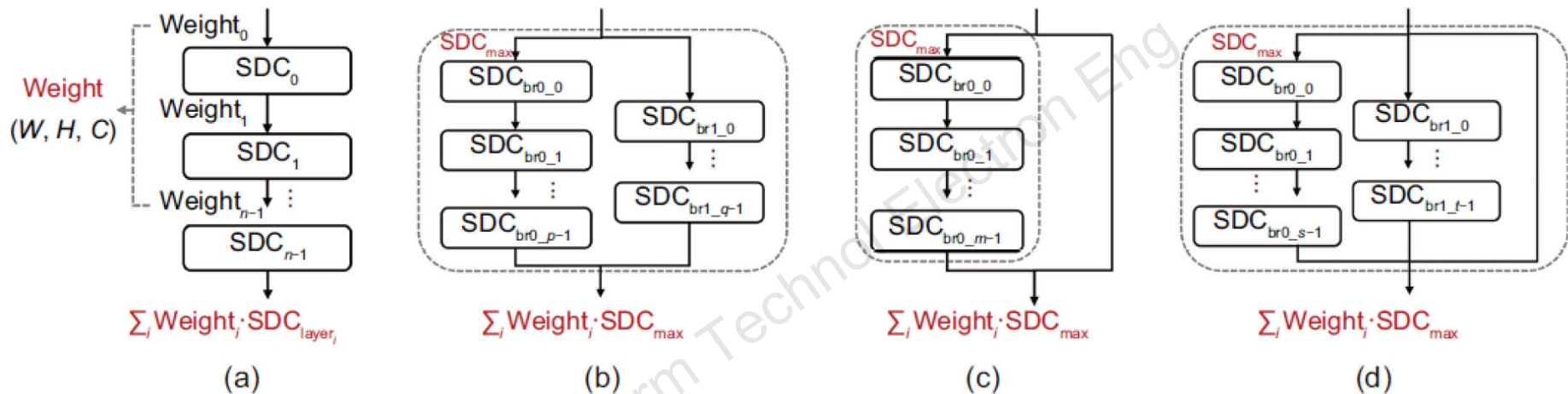
Fig. 4 Various DNN topologies: (a) sequential structure; (b) branch topology 1 (both branches have hidden layers); (c) branch topology 2 (one branch contains hidden layers); (d) branch topology 3 (some branches have hidden layers and some do not)
