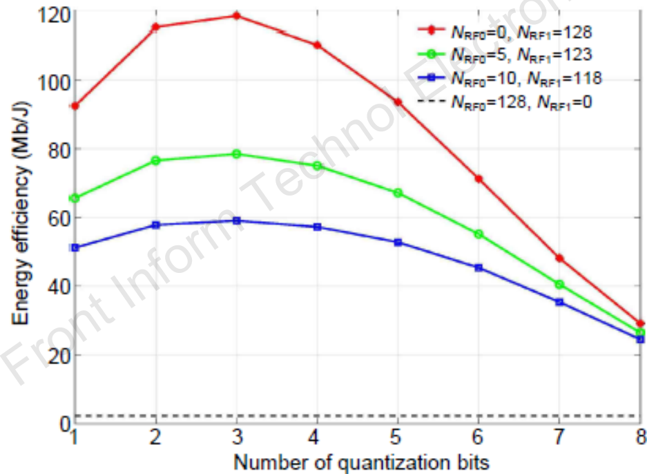
Fig. 8 Energy efficiency of multi-cell mixed-ADC mmWave massive MIMO systems over different numbers of ADC quantization bits with N_r=256 and N_{RF0}=0, 5, 10, 128
