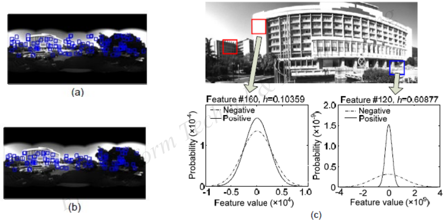
Fig. 2 Illustration of the adaptive compressive feature
