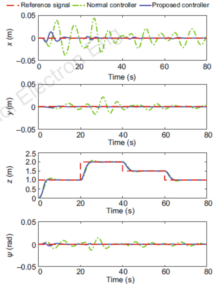
Fig. 2 Tracking performance of the different controllers in scenario 1
