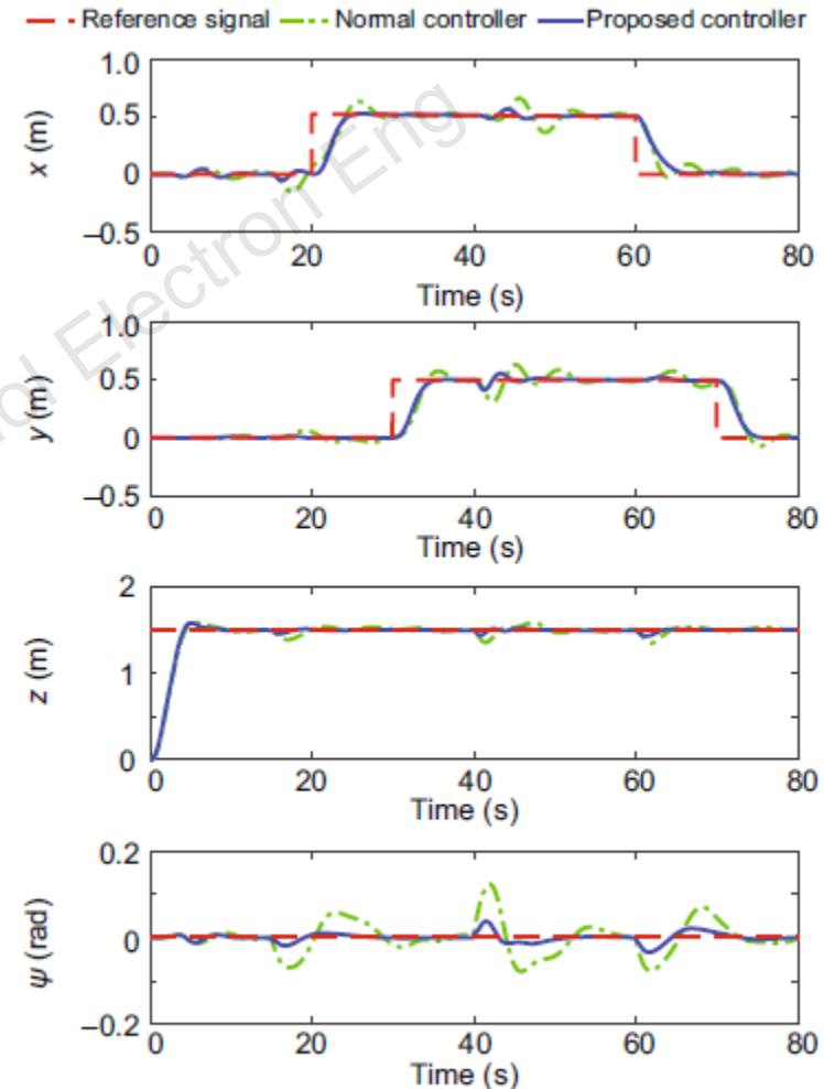
Fig. 7 Tracking performance of the different controllers in scenario 3
