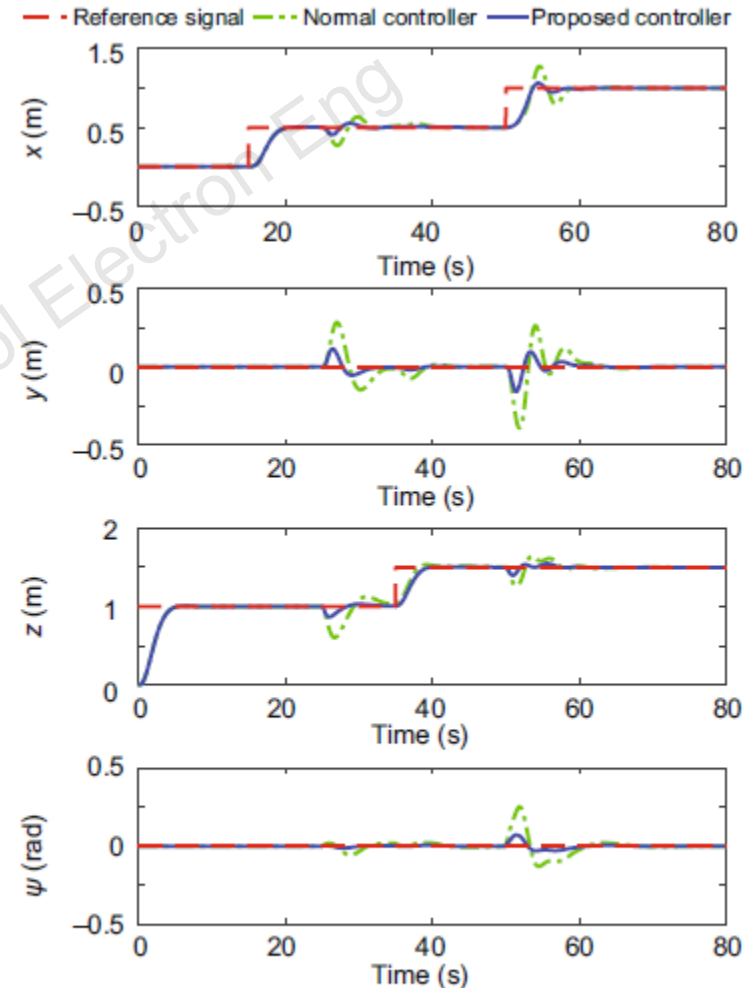
Fig. 4 Tracking performance of the different controllers in scenario 2
