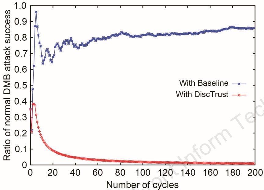
Normal diverse miner behavior (DMB) attack success ratio
