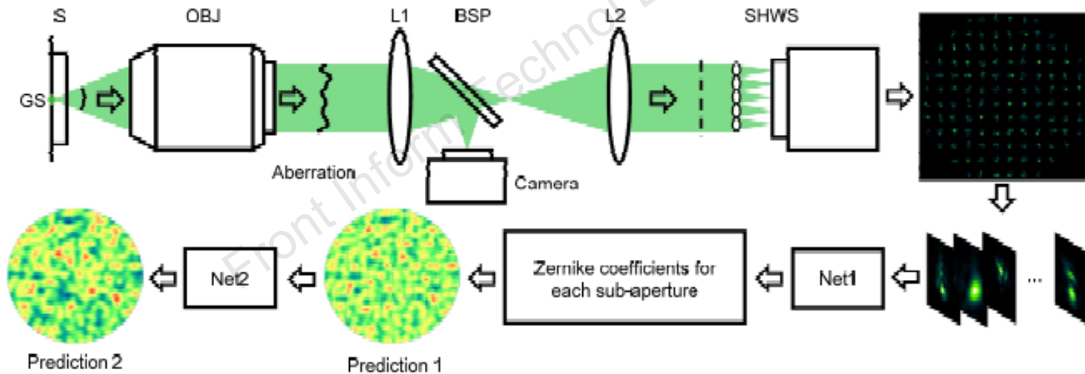
Fig. 1 Illustration of the two-step wavefront detection
