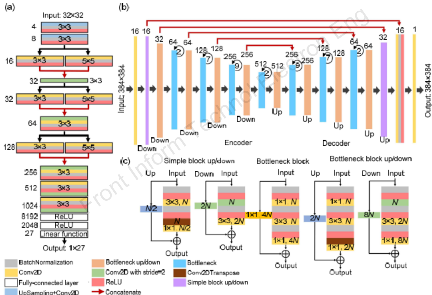
Fig. 2 Illustration of convolutional neural network architectures
