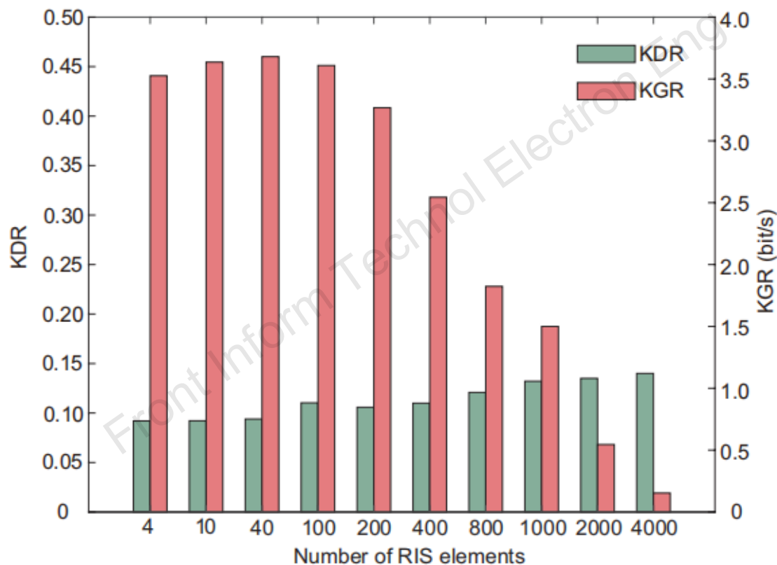
Fig. 7 Impact of RIS configuration size on KGR and KDR
