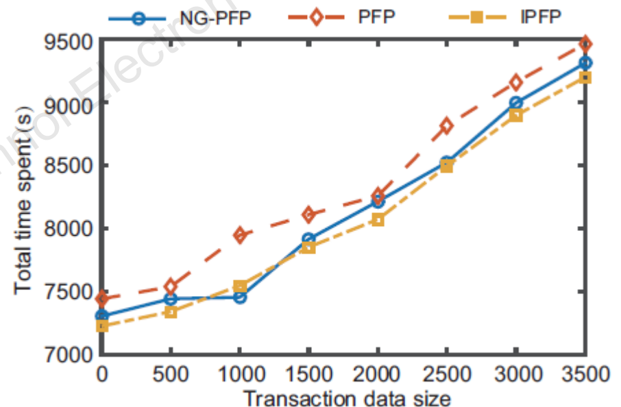
Fig. 12 Total time spent by data
