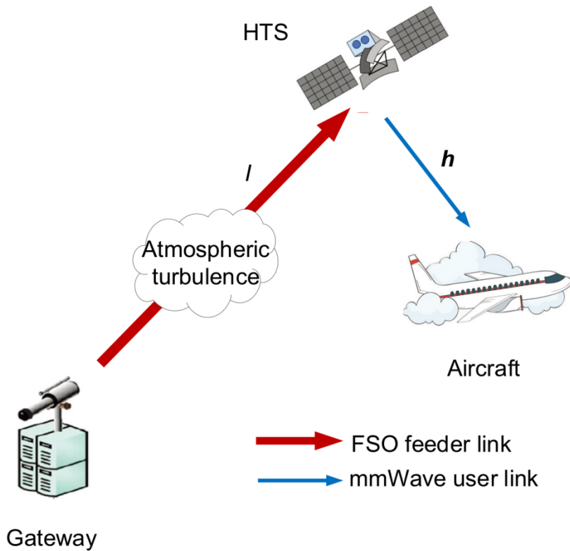
Fig. 1 System model
