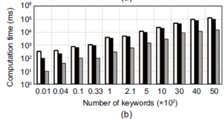
Fig. 11 Computation time of \text{Encrypt}(\cdot) : (a) mobile device; (b) computer
