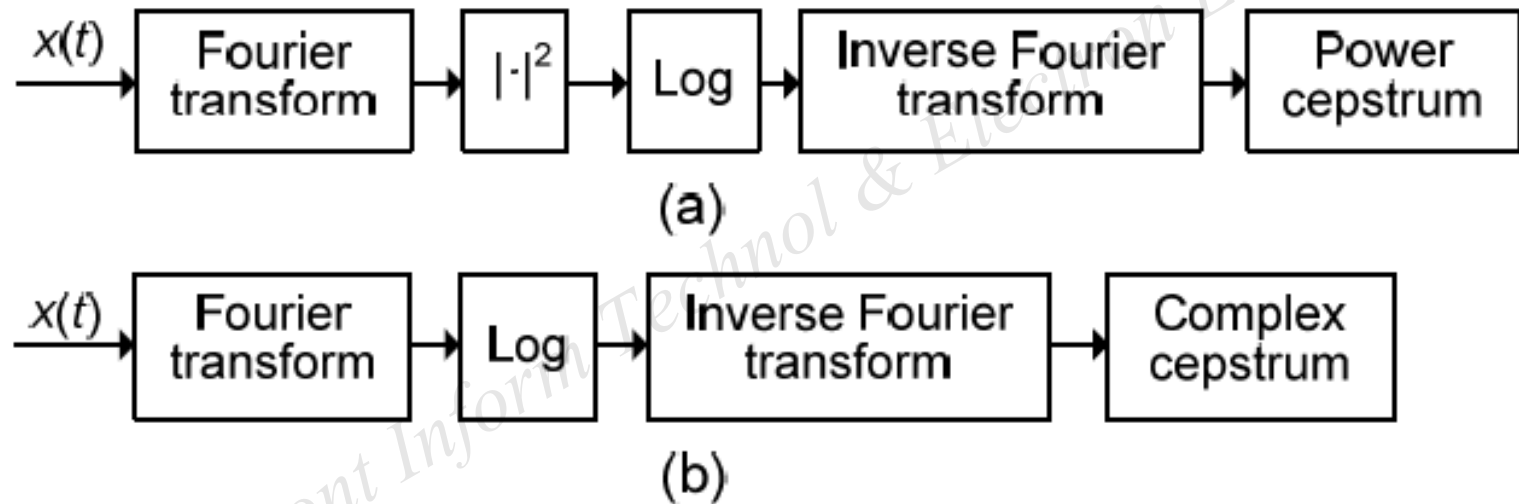
Fig. 2 Block diagrams of power (a) and complex (b) cepstrums
