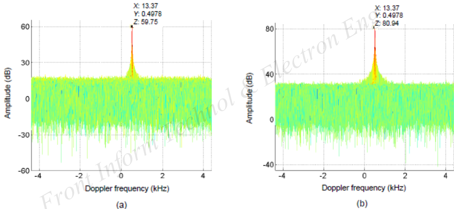
Fig. 7 Simulation results of the improved CEPMTD algorithm: (a) P=10 ; (b) P=100
