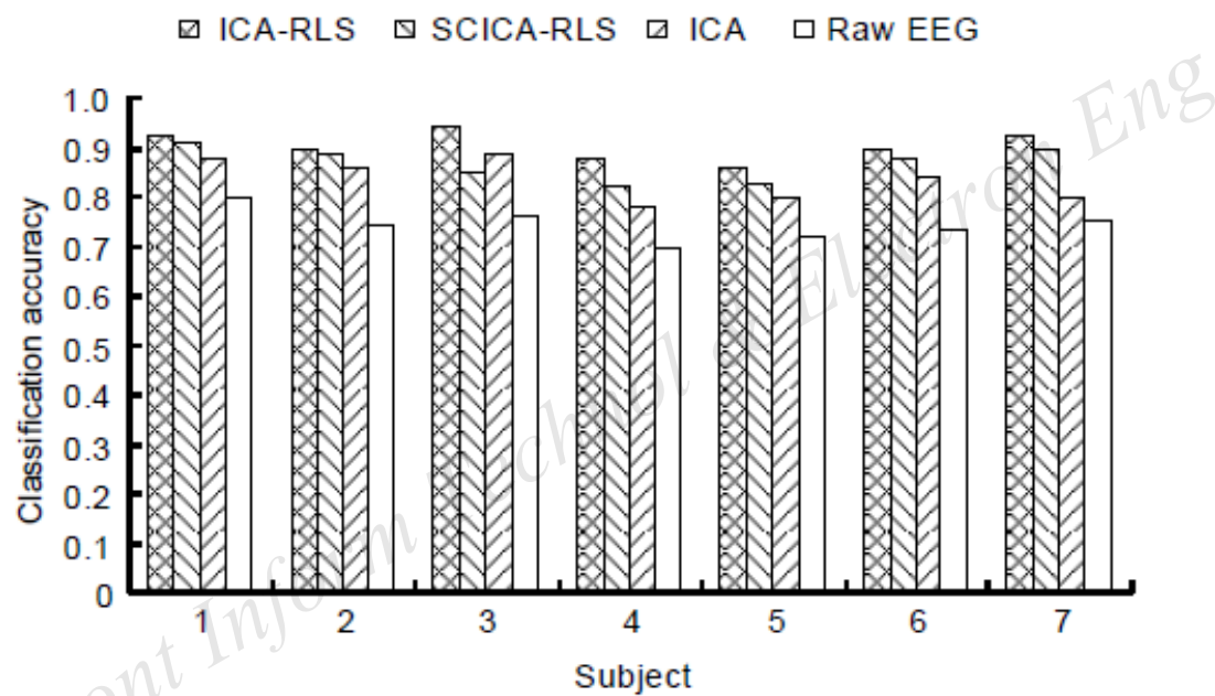
Fig. 8 Comparison of classification accuracies for different methods and subjects
