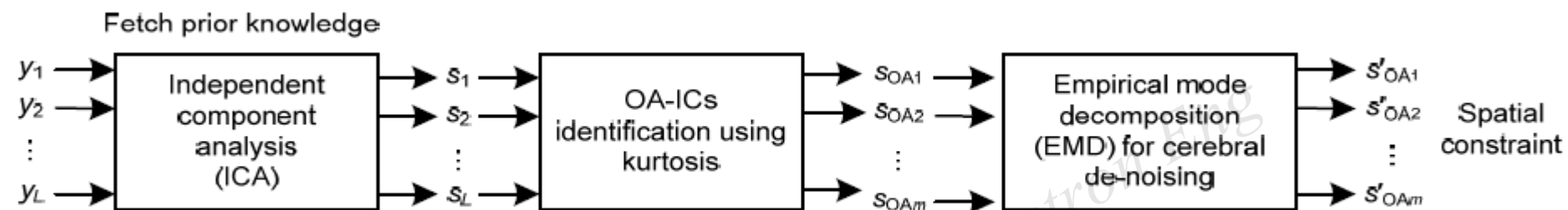
Fig. 4 Block diagram of the first stage
